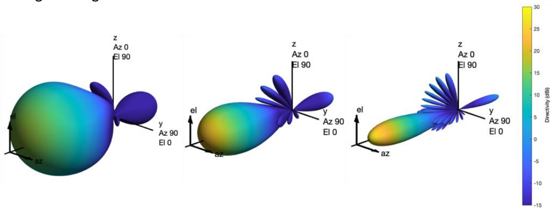
Figure 1 – The radiation pattern of the Tx antenna corresponding to (left to right) 4 \times 4 , 8 \times 8 , 16 \times 16 arrays
