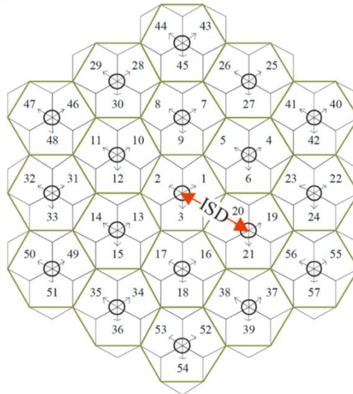
Figure 4 – Simulated Network Layout
